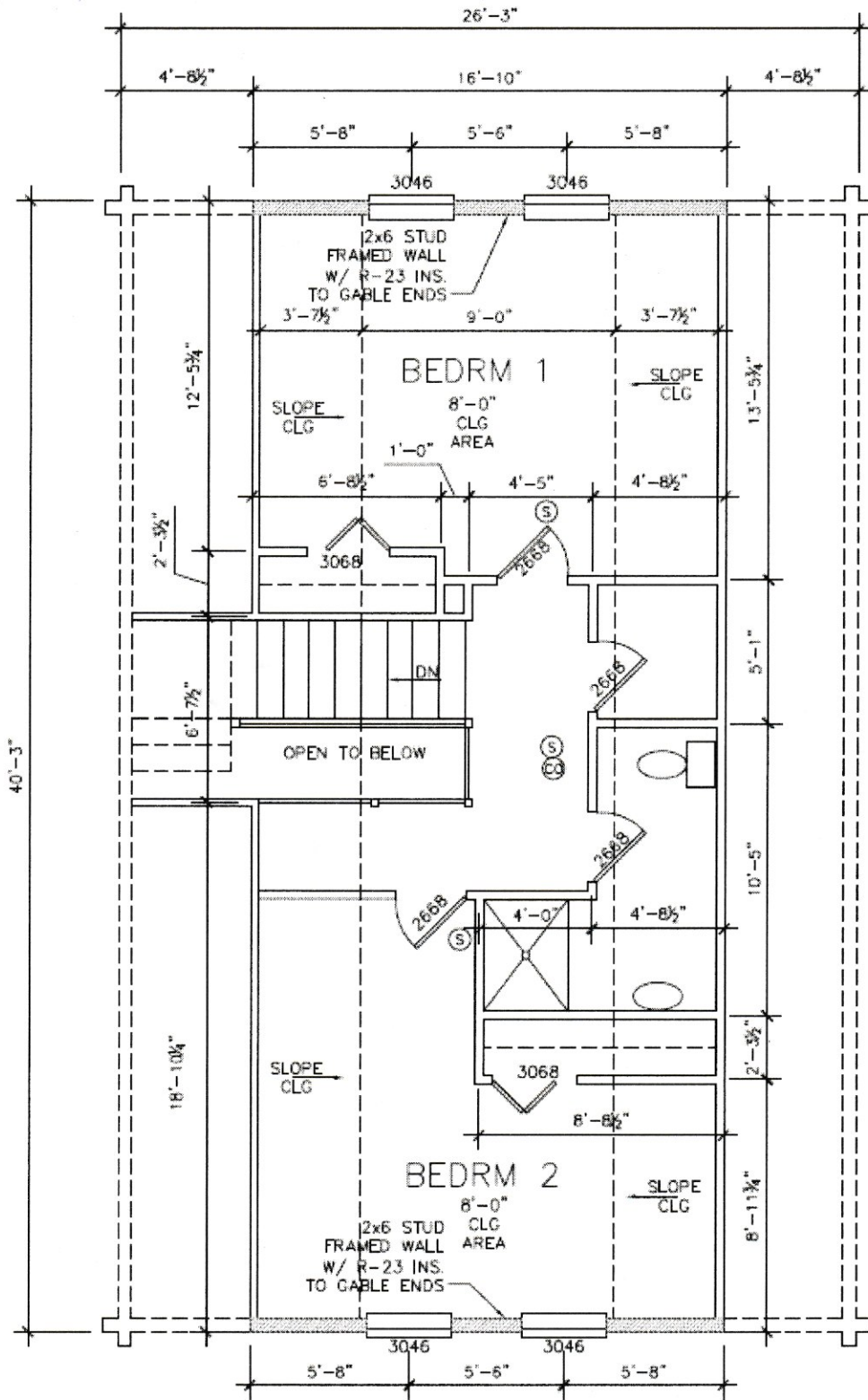
2 SECOND FLOOR PLAN C2 1/4"=1'-0"
